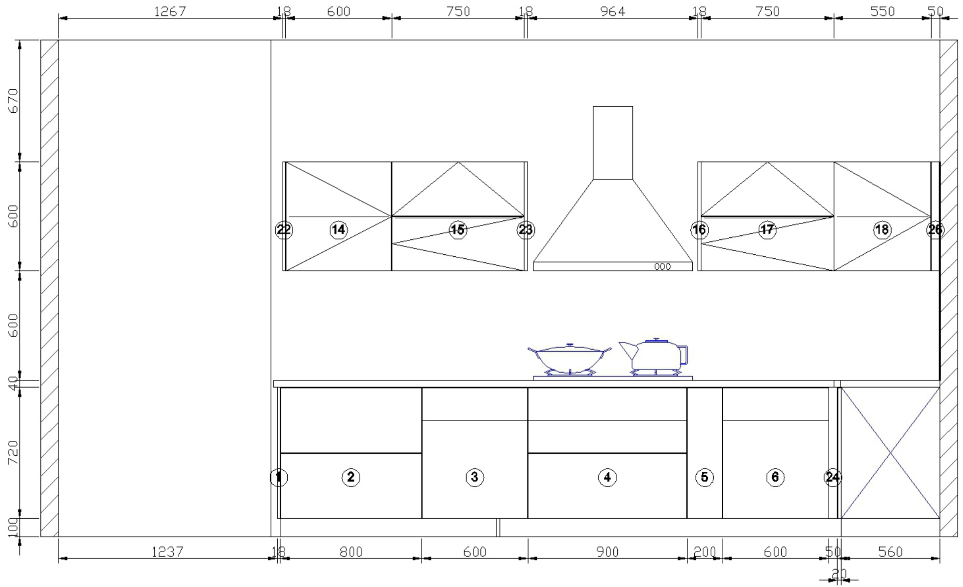
A View elevation drawing
