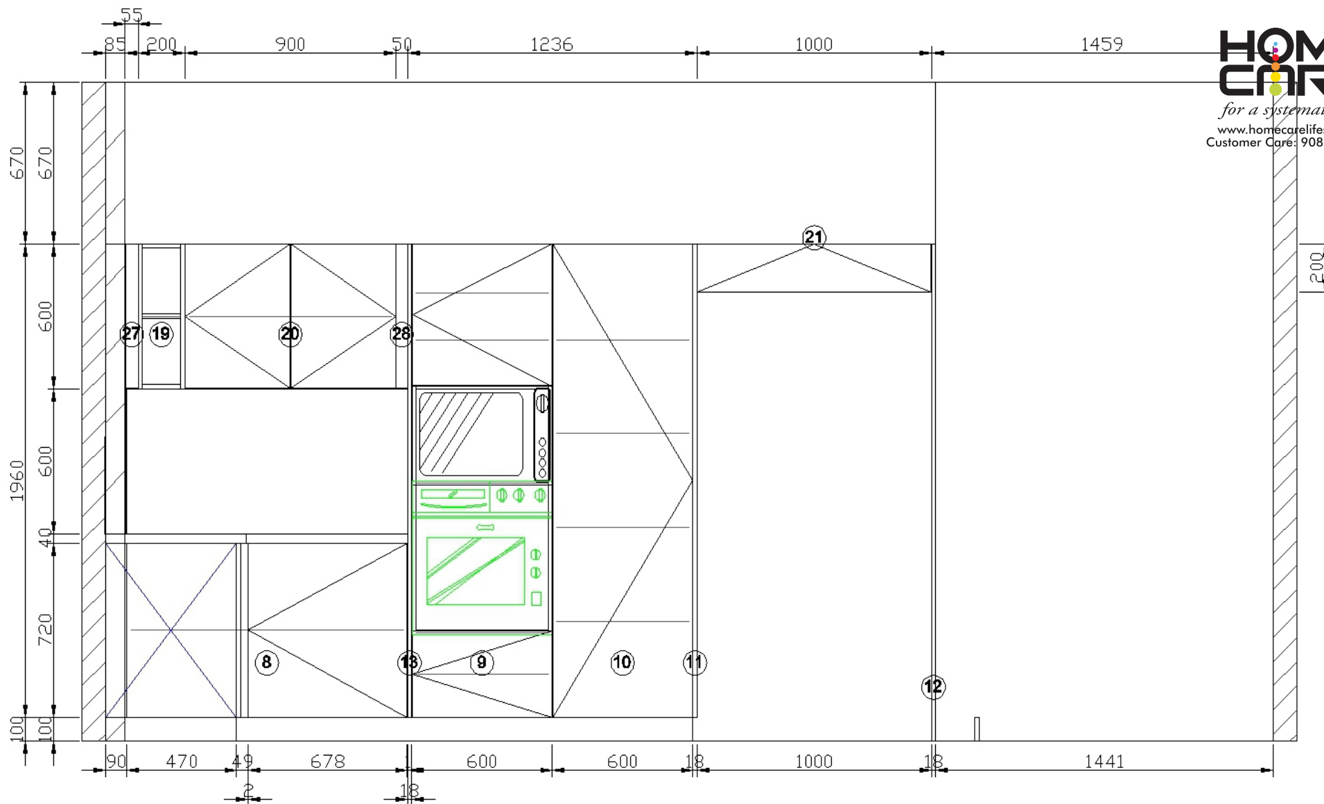
C View elevation drawing
