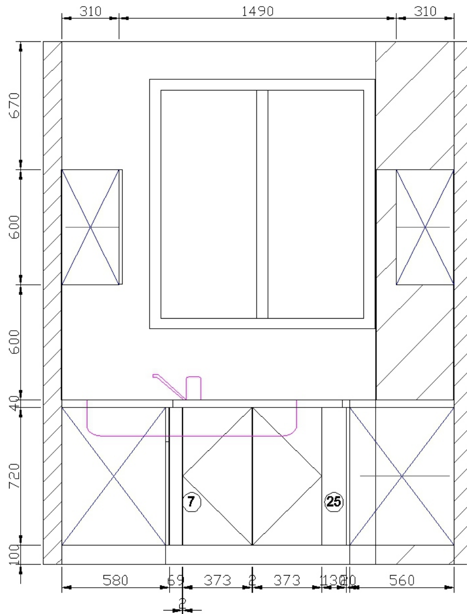
B View elevation drawing
